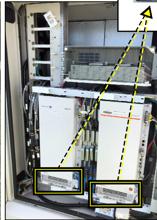
MESA 768 CABINET (INSIDE - FRONT VIEW)
