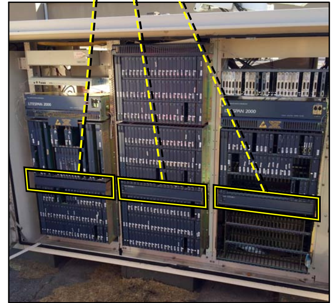
LS2000 CABINET (INSIDE - FRONT VIEW)
