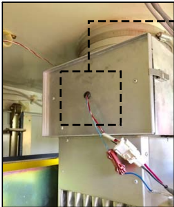
LSC-2030 CABINET HEAT STACK (OTHER SIDE OF CABINET)
