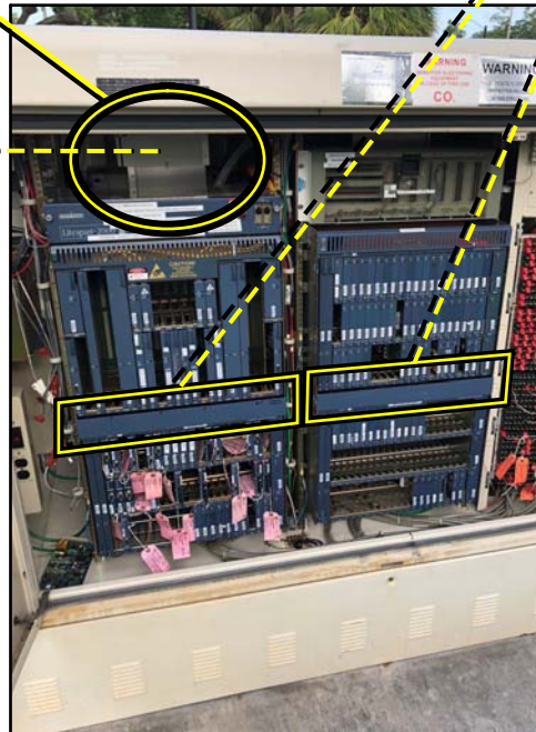
LSC-2030 CABINET (INSIDE VIEW)
