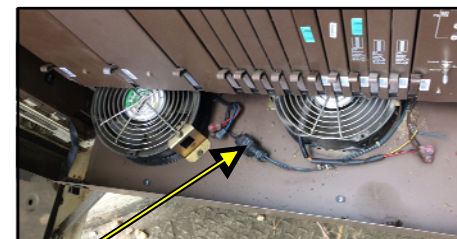
TRAY VIEW - (TF-NTOPAC) FANS w/ WEATHERPROOF (2) FANS PER TRAY
