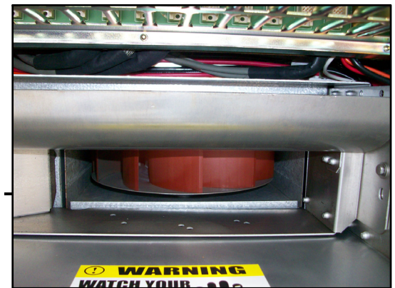
LOWER SIDE OF CABINET (BOTTOM FAN)
