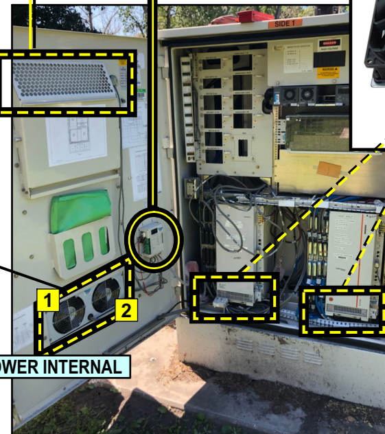
(INSIDE - HEAT EXCHANGERS, ECU & VRAD FANS)
