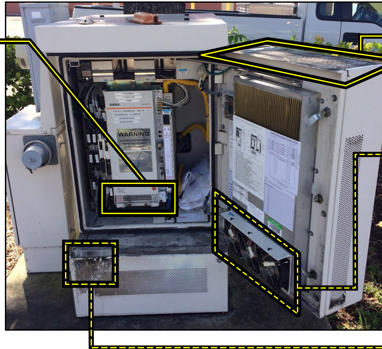
INSIDE VIEW OF CABINET
