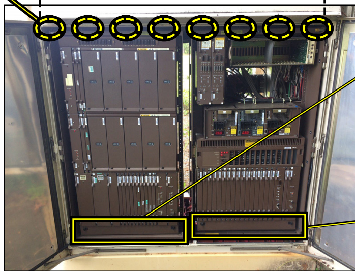
NORTEL OPAC / OPM CABINET (INSIDE VIEW)
