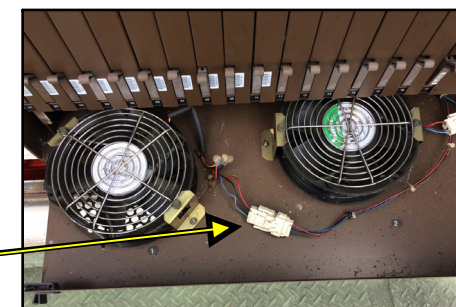
TRAY VIEW - (TF-NTOPAC-02) FANS w/ SEALED 3 PIN PLUG (2) FANS PER TRAY
