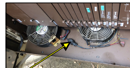
TRAY VIEW - (TF-NTOPAC) FANS w/ WEATHERPROOF PLUG (2) FANS PER TRAY
