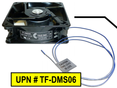
UPN # TF-DMS06 (NEW Replacement Fan) (3) FANS PER BFU
