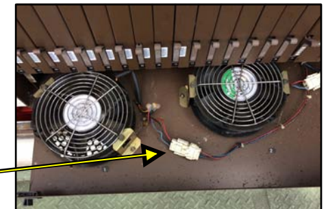
TRAY VIEW - FANS w/ SEALED 3 PIN PLUG (2) FANS PER TRAY
