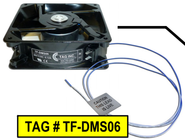
TAG # TF-DMS06 (NEW Replacement Fan) (3) FANS PER BFU
