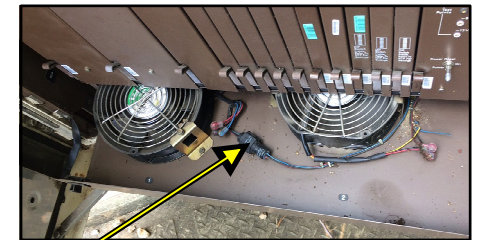
TRAY VIEW - (TF-NTOPAC) FANS w/ WEATHERPROOF PLUG (2) FANS PER TRAY
