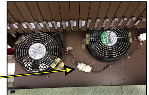
TRAY VIEW - (TF-NTOPAC-02) FANS w/ SEALED 3 PIN PLUG (2) FANS PER TRAY
