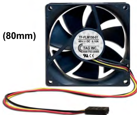
PN # TF-FLM150-01 48 Volt Replacement Fan for Fujitsu FLM 150 Fan Tray w/ 3 Wire Plug
