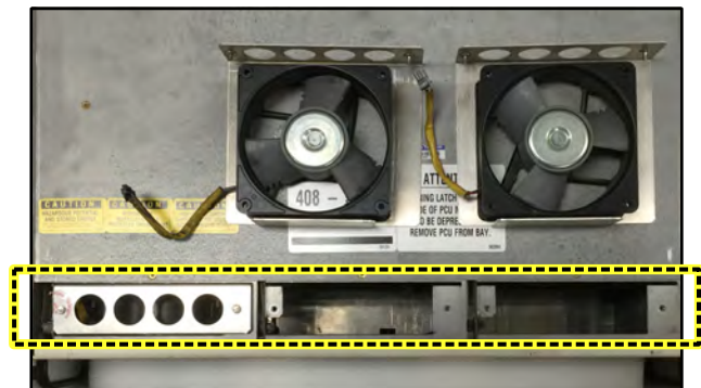
VORTEX RECTIFIER FAN UNIT w/ EXISTING FANS (V200E50 type w/ (3) separate trays)
