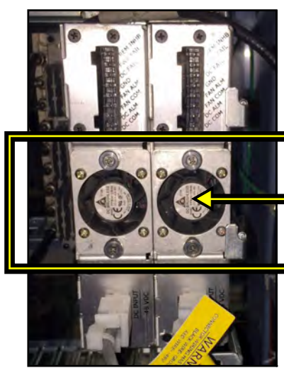
POWER SUPPLY (BACK VIEW) w/ EXISTING FANS
