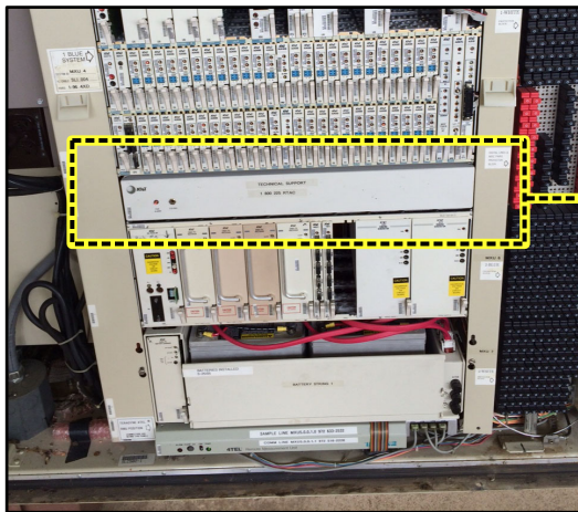
INSIDE VIEW OF 80A/D CABINET
