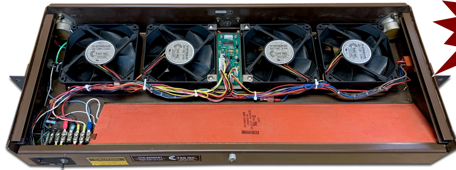
REFURBISHED DMS OPM, NT8X06AB FAN TRAY * WITH (4) NEW 48V FANS & NEW ALARM CONTROL BOARD
