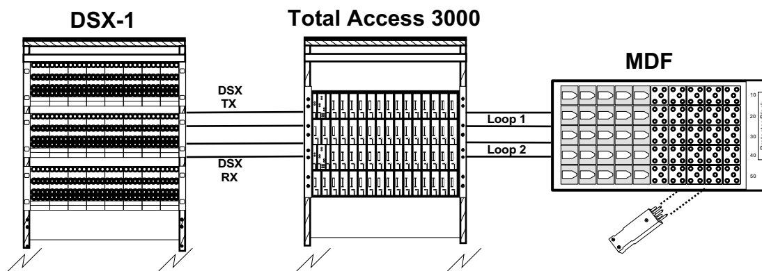
Plugs in Total Access 3000 office repeater card slots
