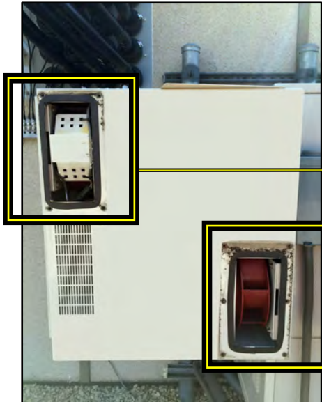
MESA XL CABINET DOOR w/ OLD FANS
