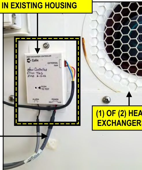
CALIX ODC-2000 CABINET (INSIDE VIEW)
