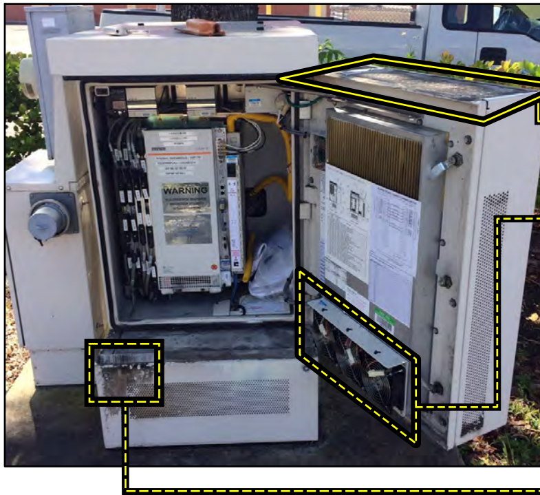
EMERSON ALP-148E CABINET
