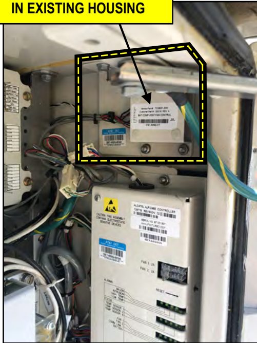
EMERSON ALP-248E / 448E CABINET (INSIDE VIEW)
