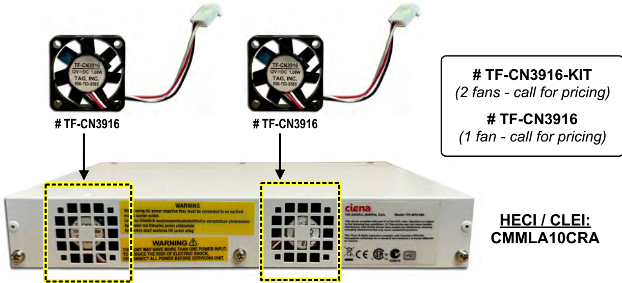
CIENA 3916 SERVICE DELIVERY SWITCH (fans only - use in existing module)
