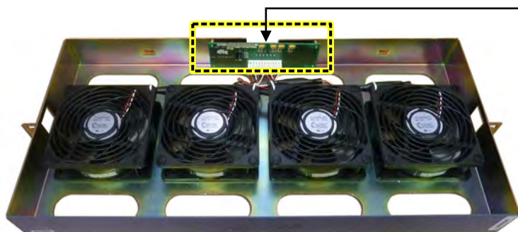
KIT SHOWN INSTALLED IN EXISTING DFA FAN TRAY * *(DFA FAN TRAY IS NOT INCLUDED)
