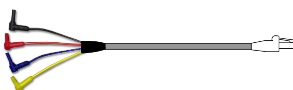
HST3000 to RJ48C - (T1), (6') (RJ48 Pins 1,2,4,5) Part #: ACT-400148BY
