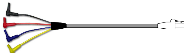
HST3000 to RJ48S - (DDS), (6') (RJ48 Pins 1,2,7,8) Part #: ACT-400148SBY
