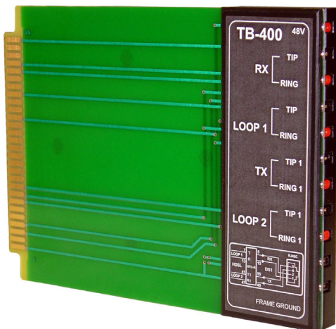
TB-400 200/400 Shelf HDSL Test Board (w/ Pin Jacks)
