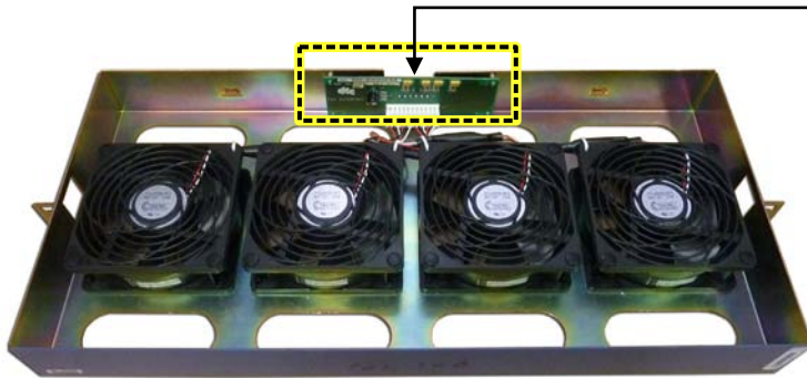
KIT SHOWN INSTALLED IN EXISTING DFA FAN TRAY * *(DFA FAN TRAY IS NOT INCLUDED)
