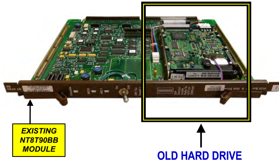
NORTEL DMS-10 NT8T90BB MODULE w/ Hard Drive (w/ "MOVING PARTS")
