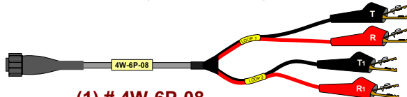
(1) # 4W-6P-08 Female Lock Plug to (4) 6P Alligator Clips, (8')
