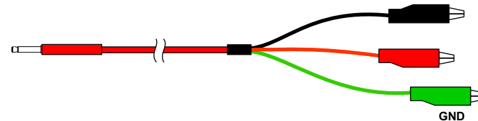
(1) PN # 400210A3RD Bantam to (3) Alligator Clips - Red, (6')
