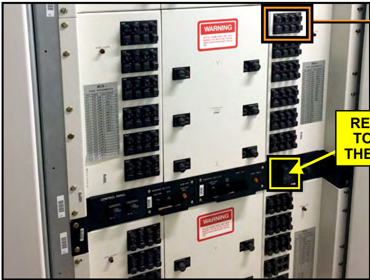
5ESS Fuse Bay Control Panel, Lucent # ED-83024-30
