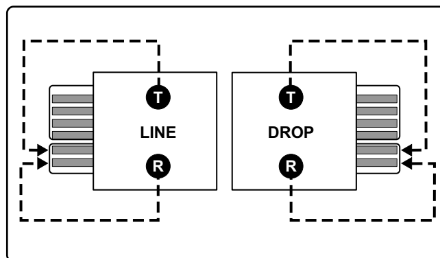
Wiring Details:
