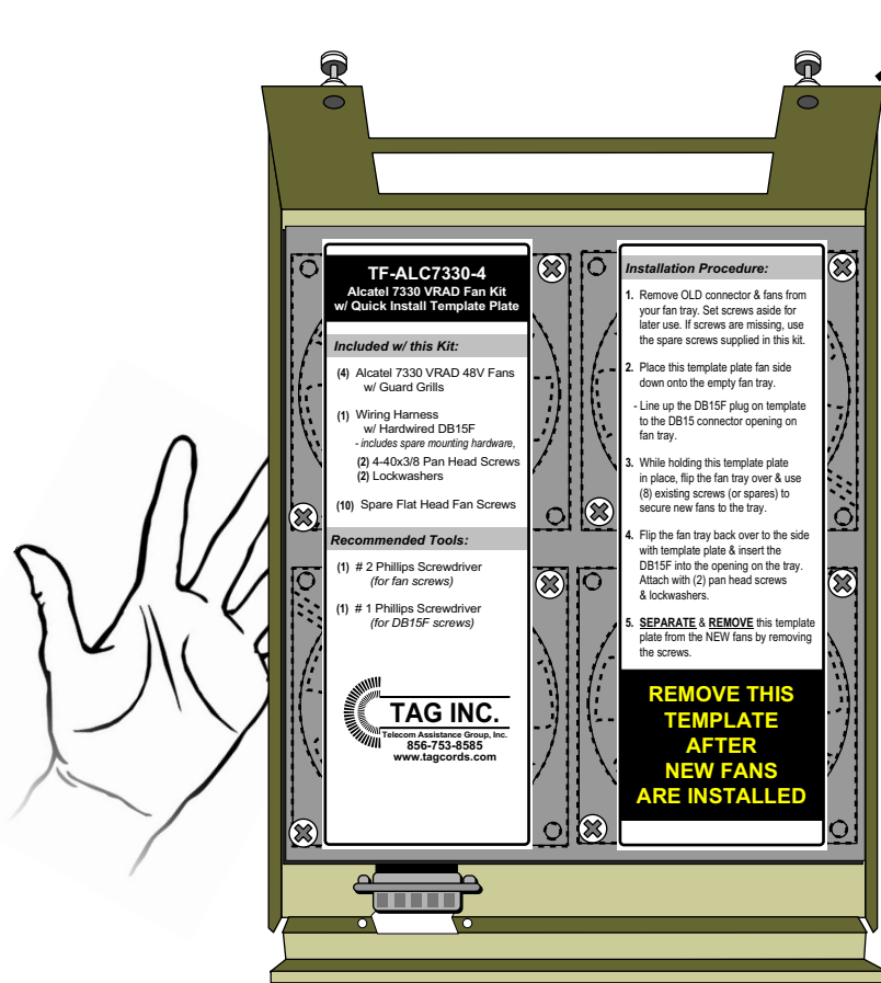
TEMPLATE PLATE w/ NEW FANS INVERTED OVER THE INSIDE OF THE TRAY
