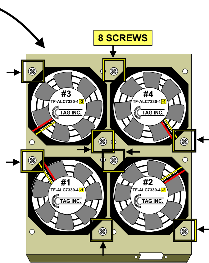
TRAY WITH NEW FANS EXTERNAL VIEW
