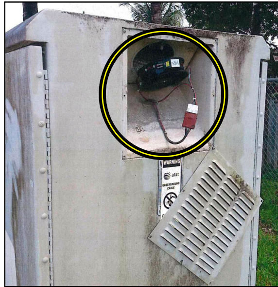
PN # TF-FUJ6200-01 48V Replacement Heat Exchanger for Fujitsu 6200 Cabinet w/ 5 Wire Plug
