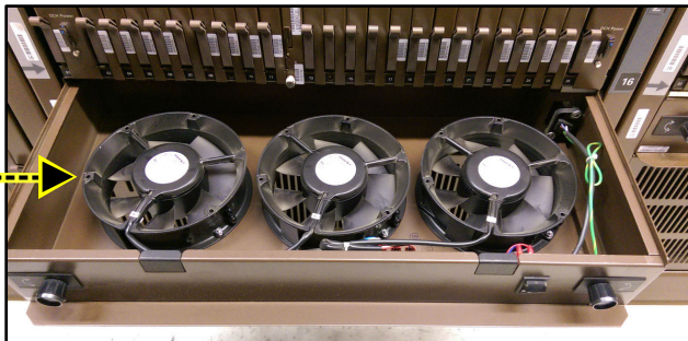
DMS-100 NTRX91AA FAN UNIT w/ EXISTING FANS
