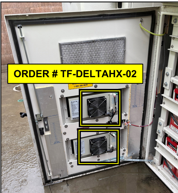
DELTA HEAT EXCHANGER (QTY OF 2 - INNER )
